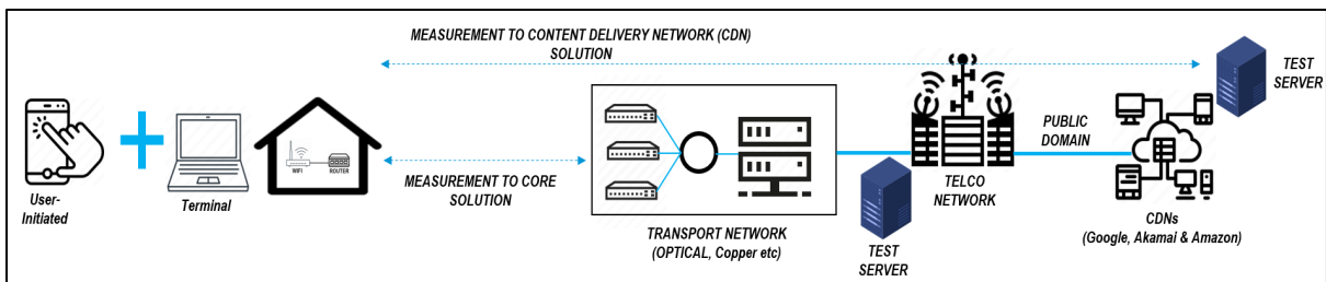
Figure 5. Fixed network measurement overview
