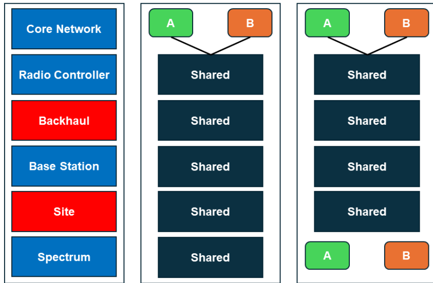
Figure D.2. MOCN and MORAN Infrastructure sharing
