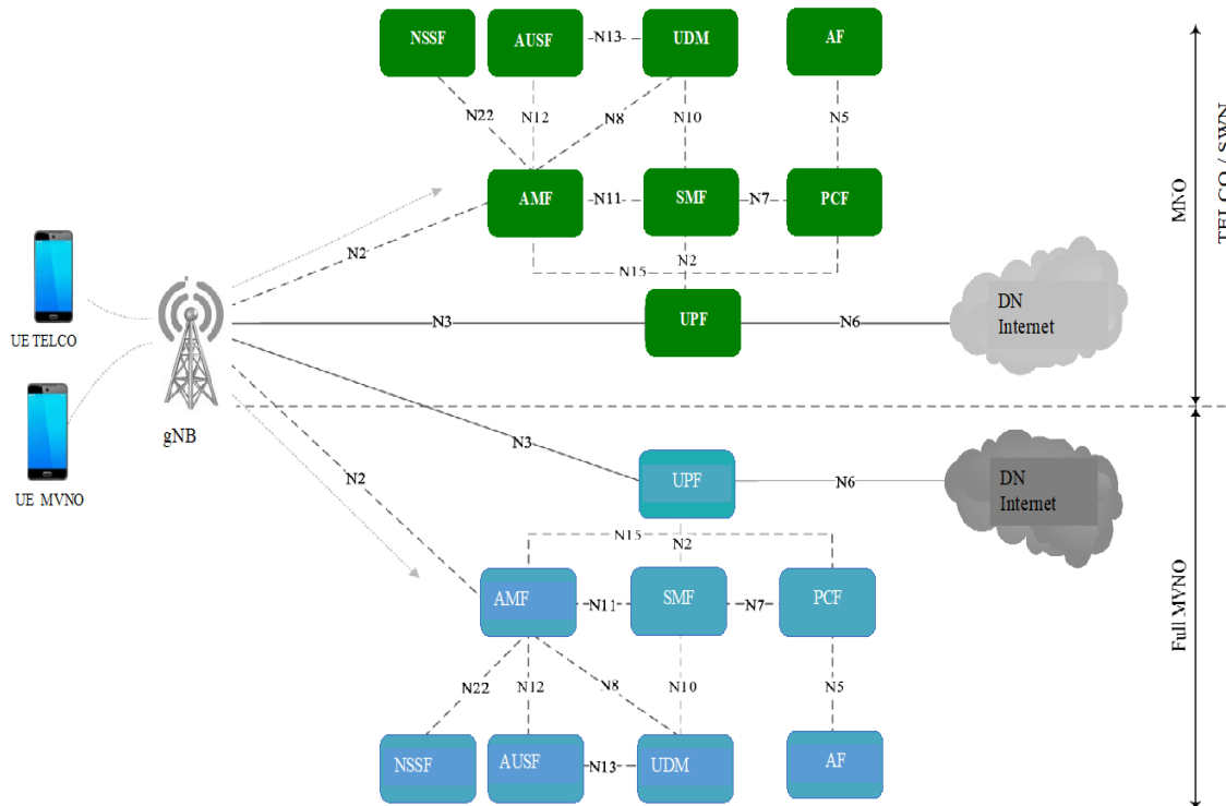
Figure 9. 5G MVNO using MOCN based on 5G standalone E2E network architecture
