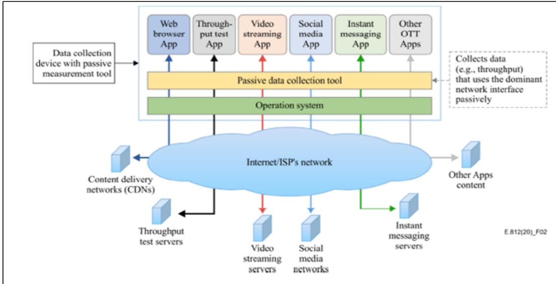
Figure 2. Passive data collection from a mobile network
