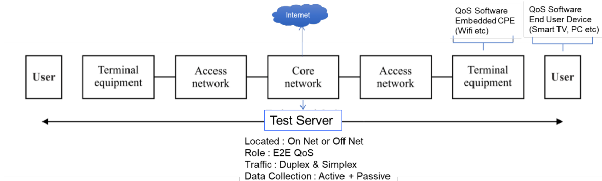
Figure 10. Fixed network set up scenario
