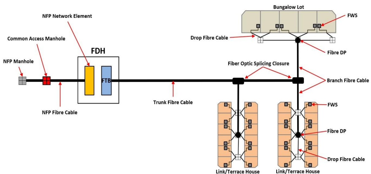
Figure 58. Cabling and network elements for strata development area
