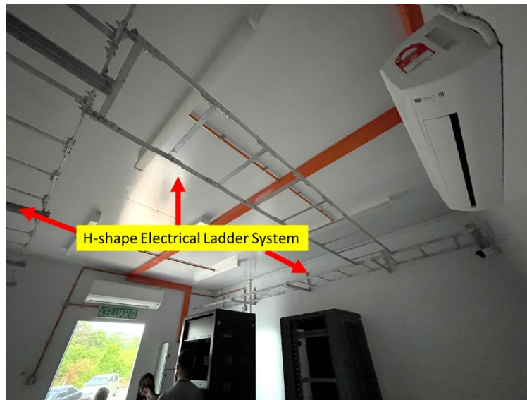
Figure 11. Sample of electrical ladder system
