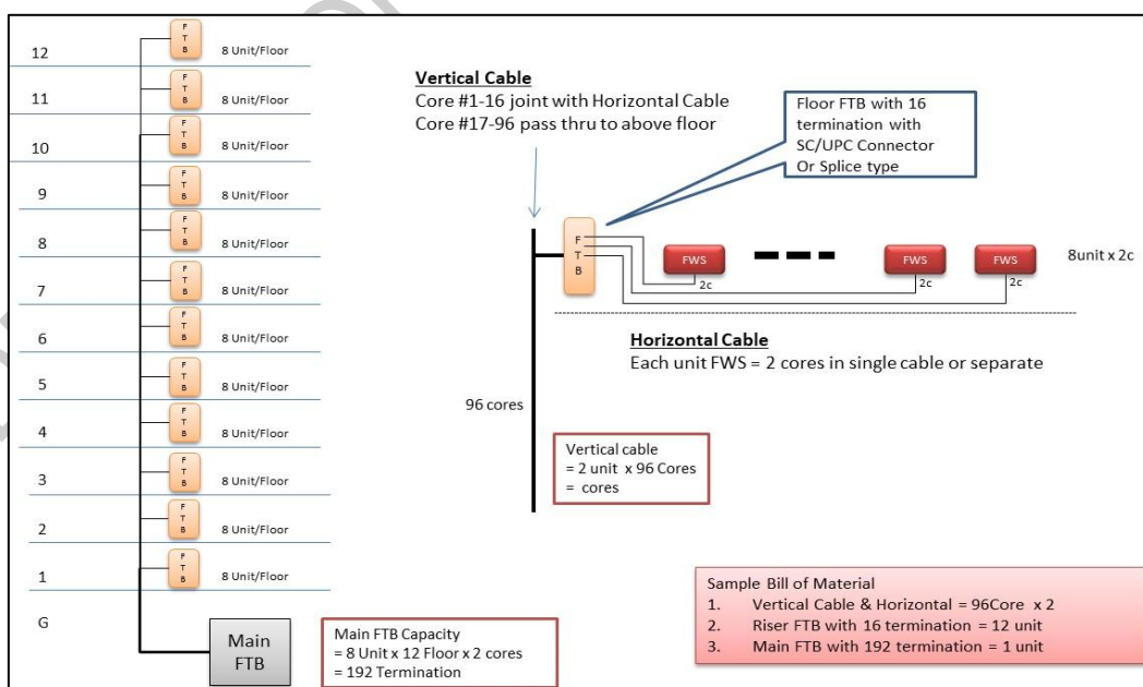
Figure 52. High-capacity vertical cable (cabling design 1)
