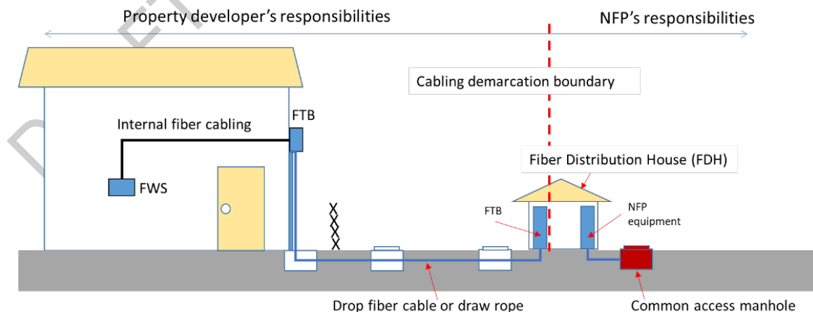
Figure 41. Cabling distribution and demarcation for landed strata
