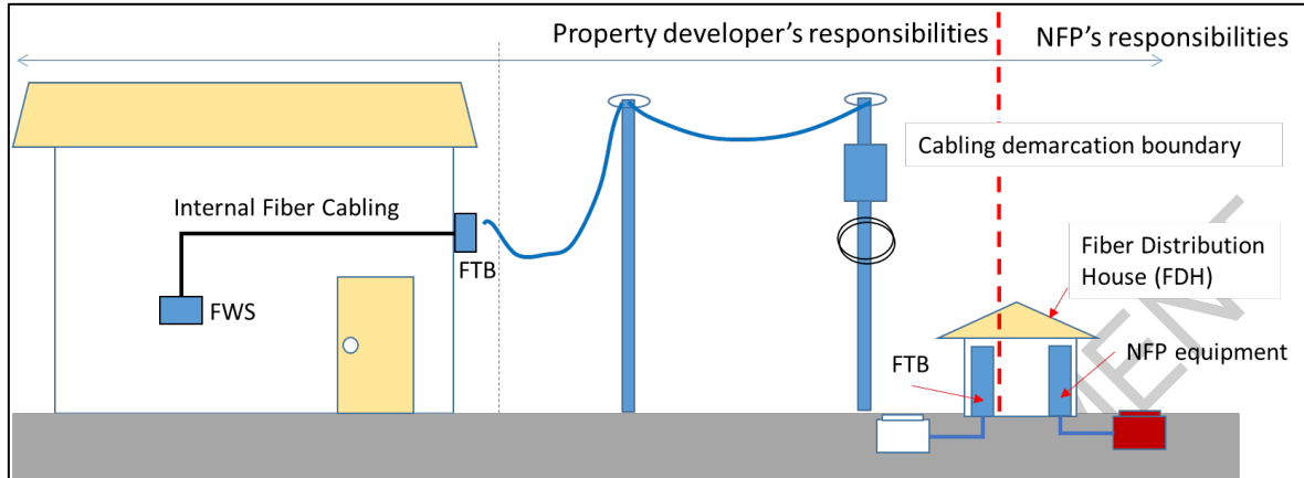
Figure 43. Strata SDU cabling demarcation boundary for pole type
