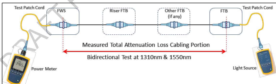
Figure 73. Power meter and light source testing method
