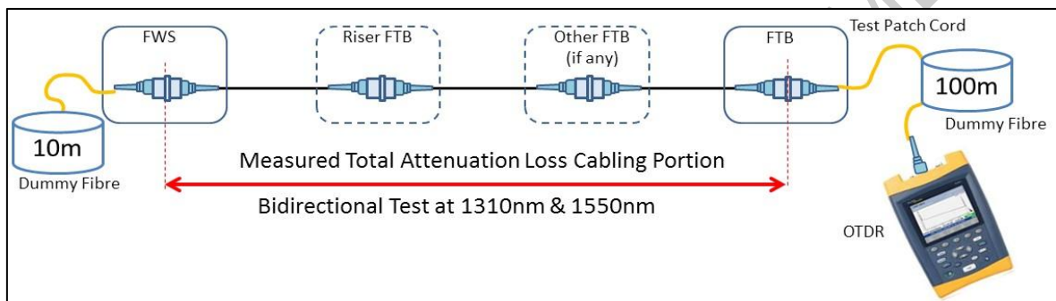
Figure 72. OTDR testing method
