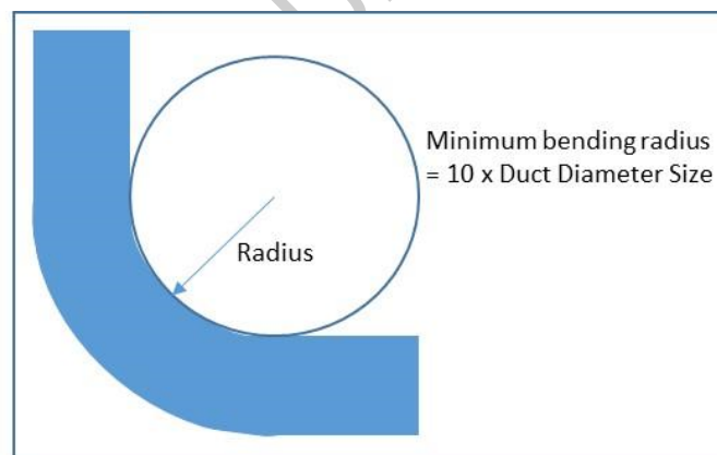
Figure 23. Duct bending radius
