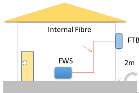
Figure 15. FTB locations for landed SDU
