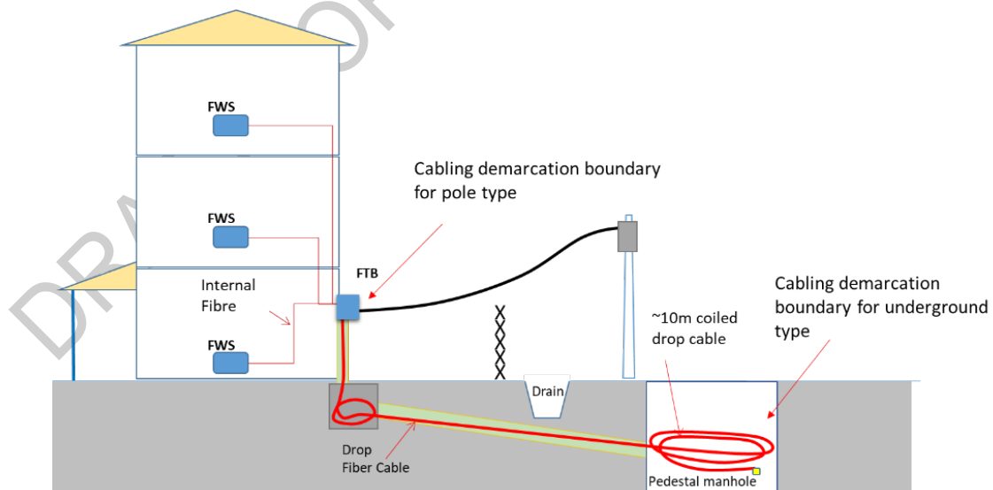
Figure 47. Cabling for town house type
