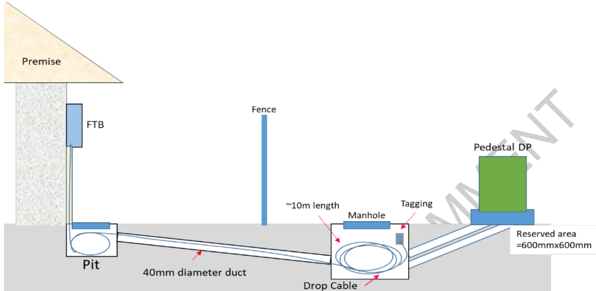
Figure 46. Connection of underground drop fibre
