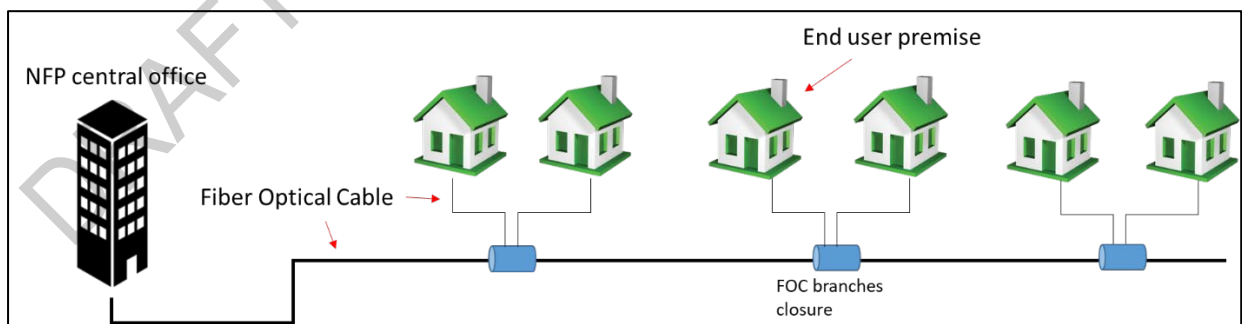
Figure 2. P2P fibre network design
