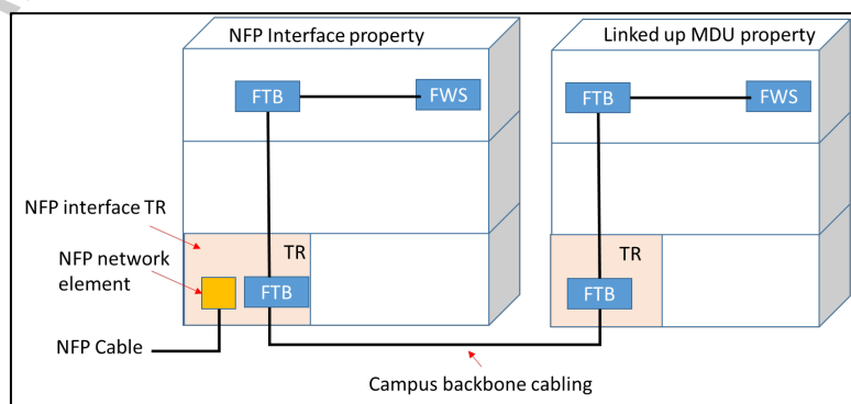
Figure 51. Campus backbone cabling
