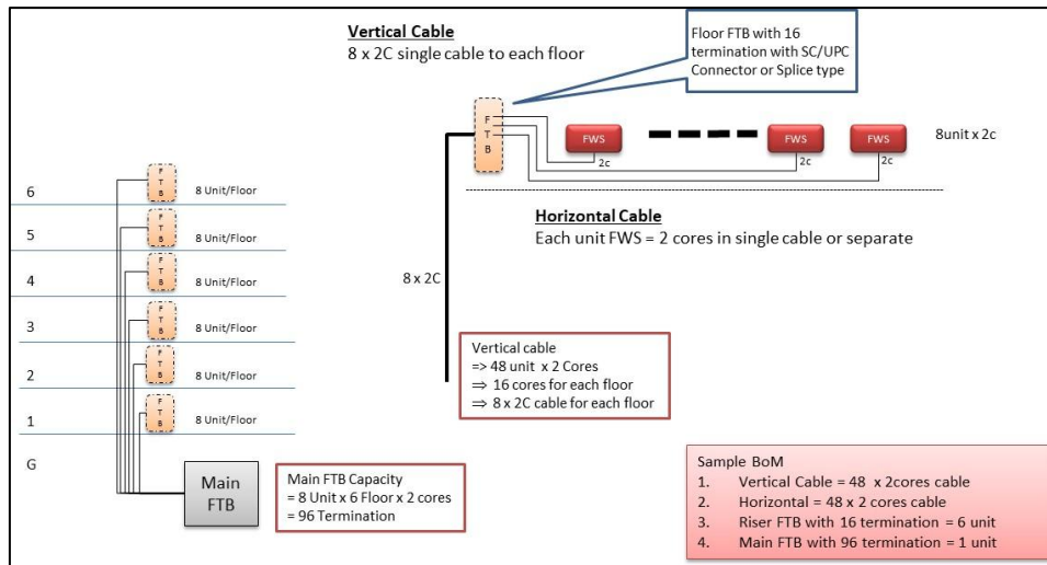
Figure 55. Single cable directly to premise unit (cabling design 4)
