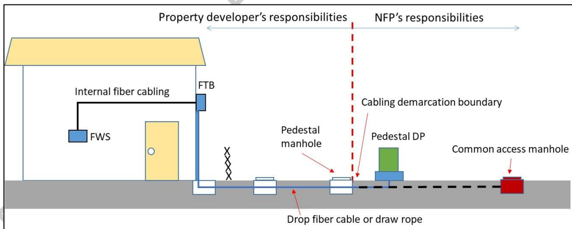
Figure 44. Non-strata SDU cabling demarcation boundary for underground type
