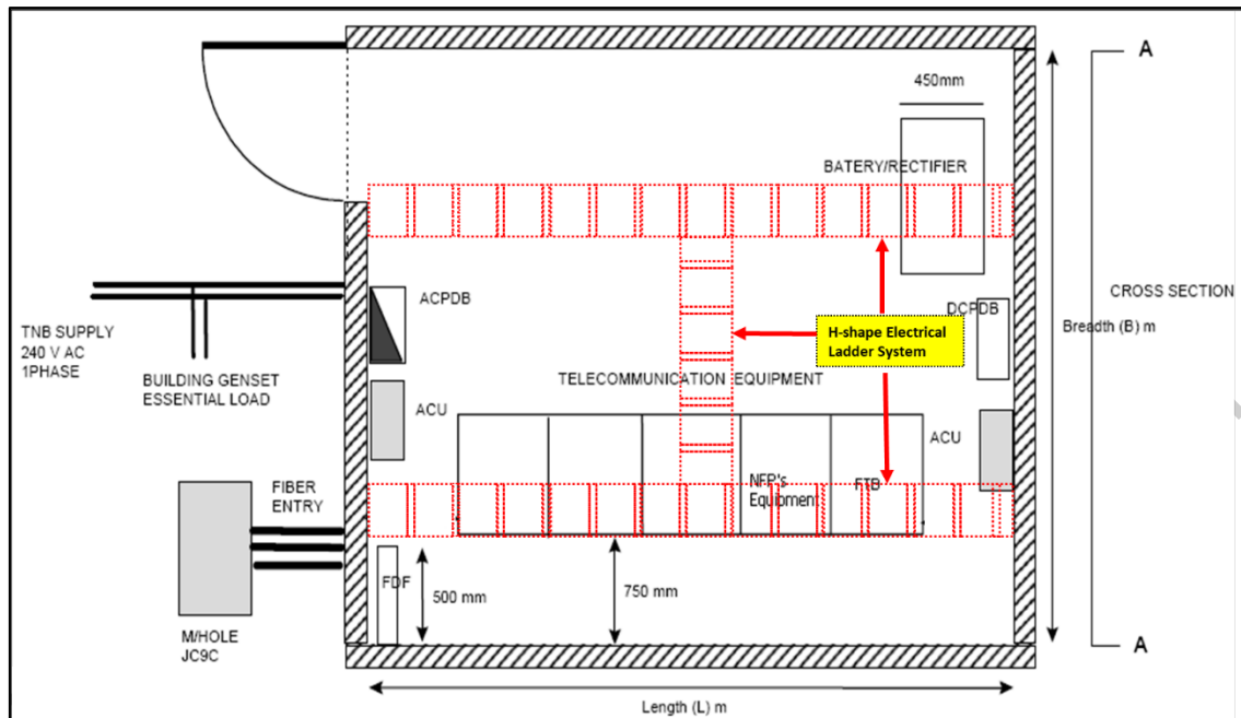
Figure 9. TR arrangement
