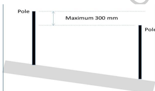
Figure 39. Non-flat ground pole installation
