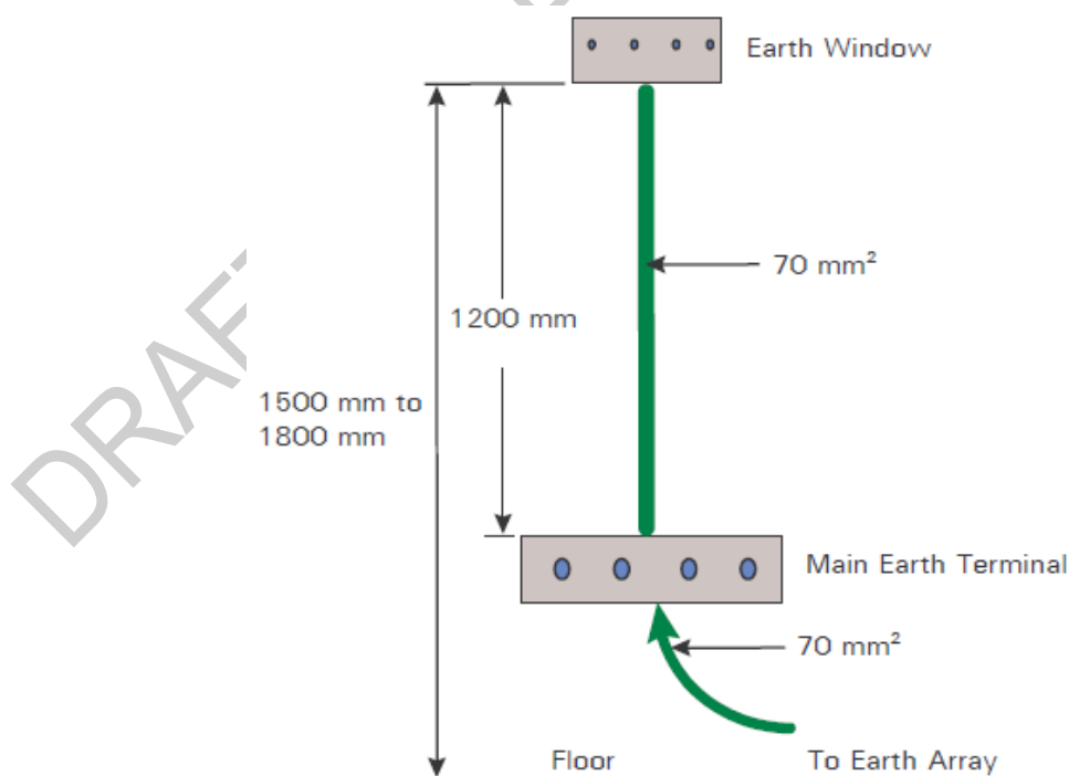
Figure 8. Grounding system termination
