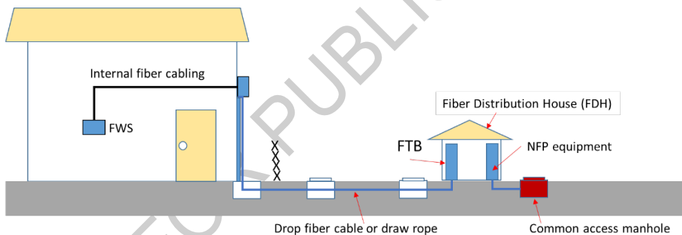
Figure 16. FTB locations for strata SDU
