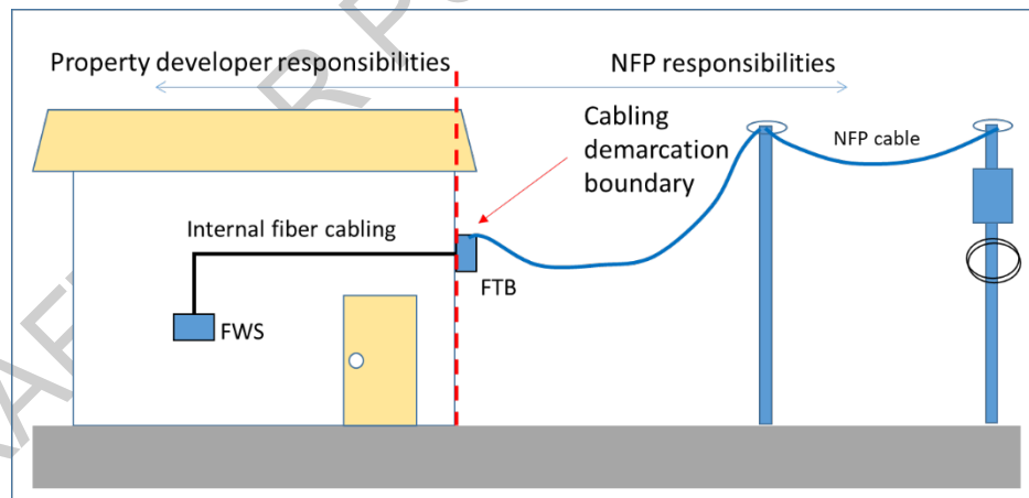
Figure 42. Non-strata SDU cabling demarcation boundary for pole type
