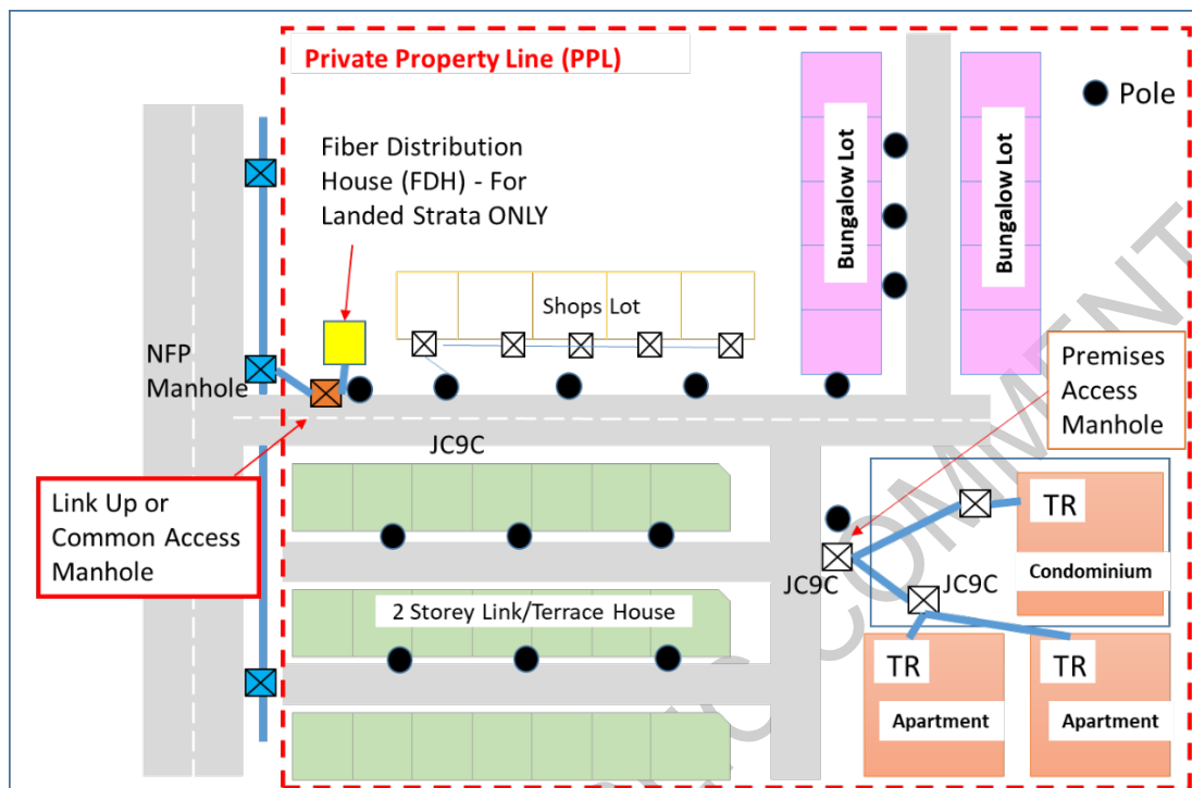
Figure 36. Pole distribution for connection via NFP's underground infrastructure
