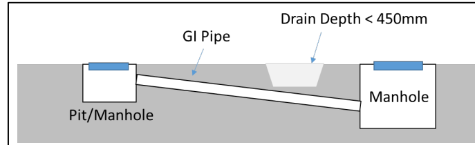
Figure 26. Ducting installation under the drain
