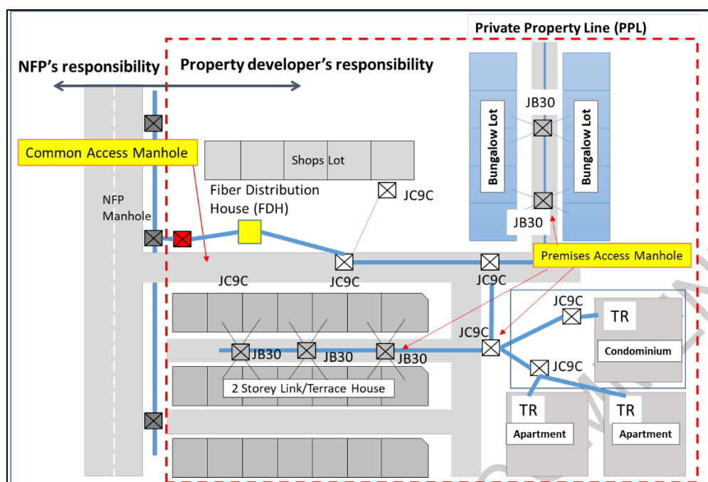
Figure 7. Strata development area infrastructure demarcation
