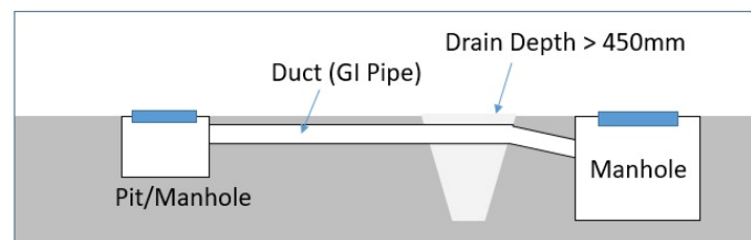
Figure 27. Ducting installation through the drain
